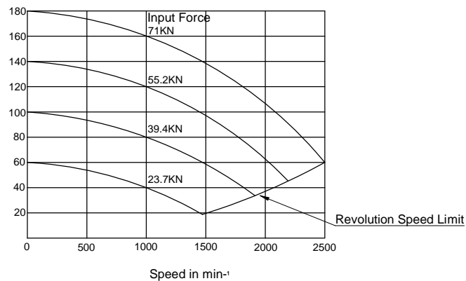
Gripping Characteristic Graph For B-15A8
