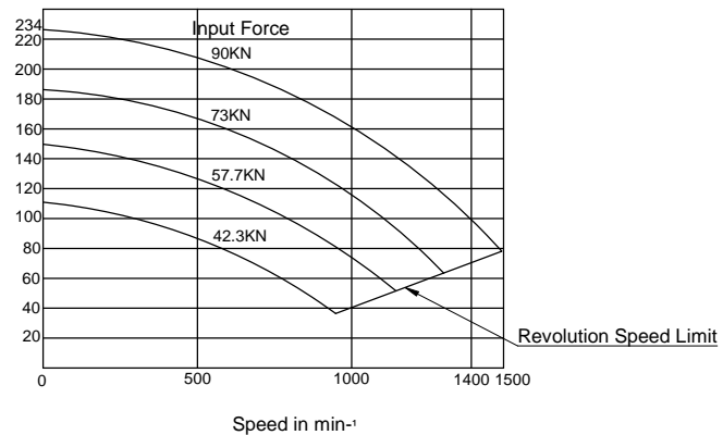
Gripping Characteristic Graph For B-24A15
