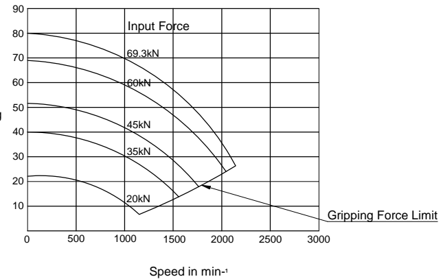
Gripping Characteristic Graph For BL-212A8
