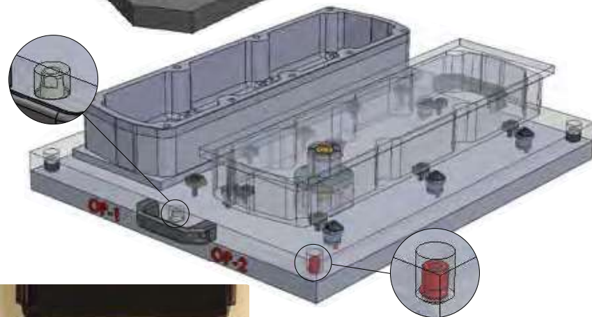
Heavy Wall Loc-Down® Bushing Part No. 11520
