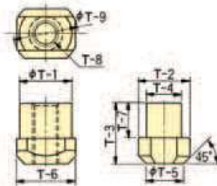
Ref. DWG. 4
