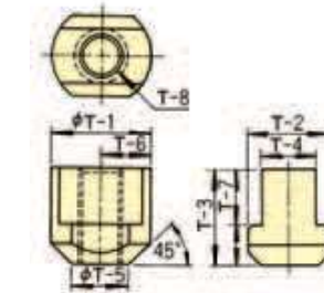
Ref. DWG. 3
