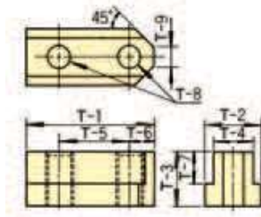
Ref. DWG. 1
