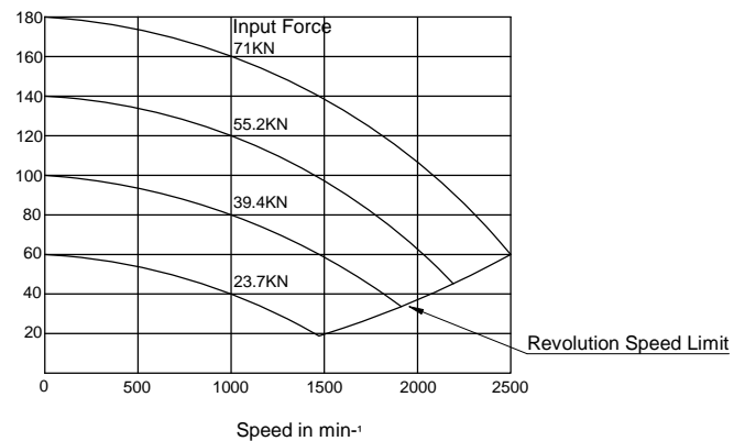
Gripping Characteristic Graph For B-15A11
