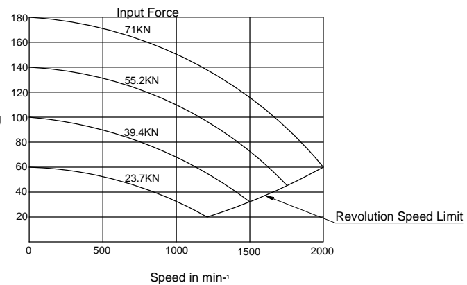
Gripping Characteristic Graph For B-18A11
