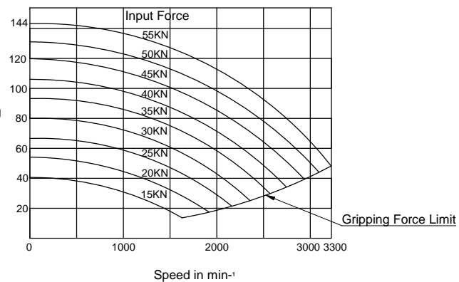
Gripping Characteristic Graph For B-212A8
