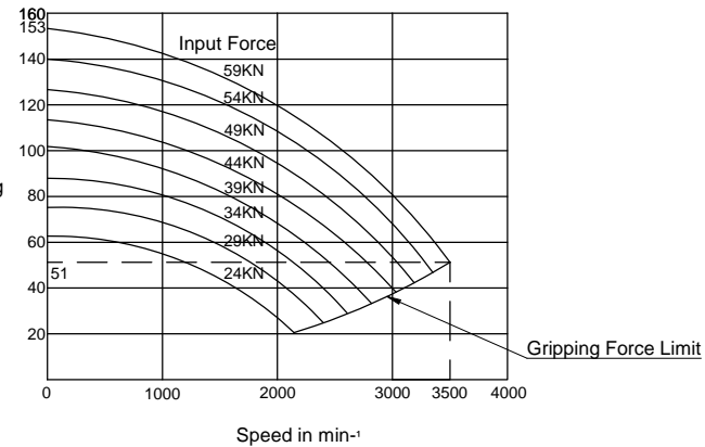
Gripping Characteristic Graph For BB-212A8
