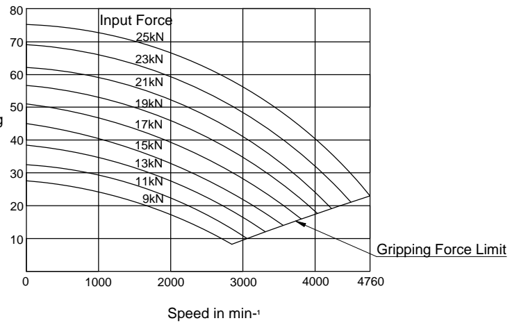
Gripping Characteristic Graph For N-08A6
