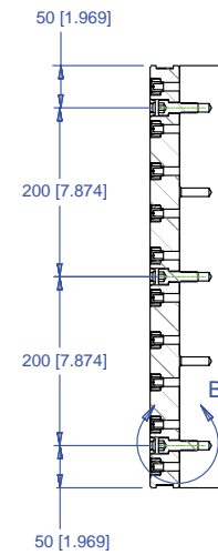
DETAIL B
